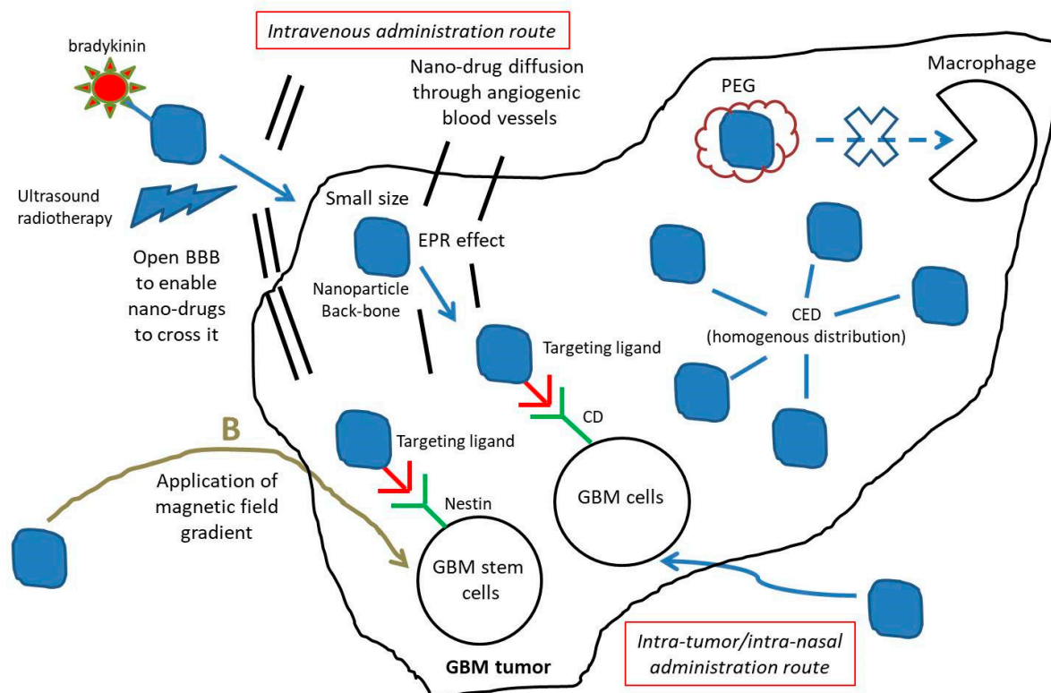
Figure 2. A schematic figure showing the various mechanisms by which anti-GBM nano-drugs can target the GBM tumor.
