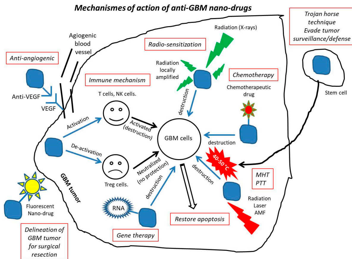
Figure 3. A schematic figure presenting the various mechanisms of action of anti-GBM drugs.
