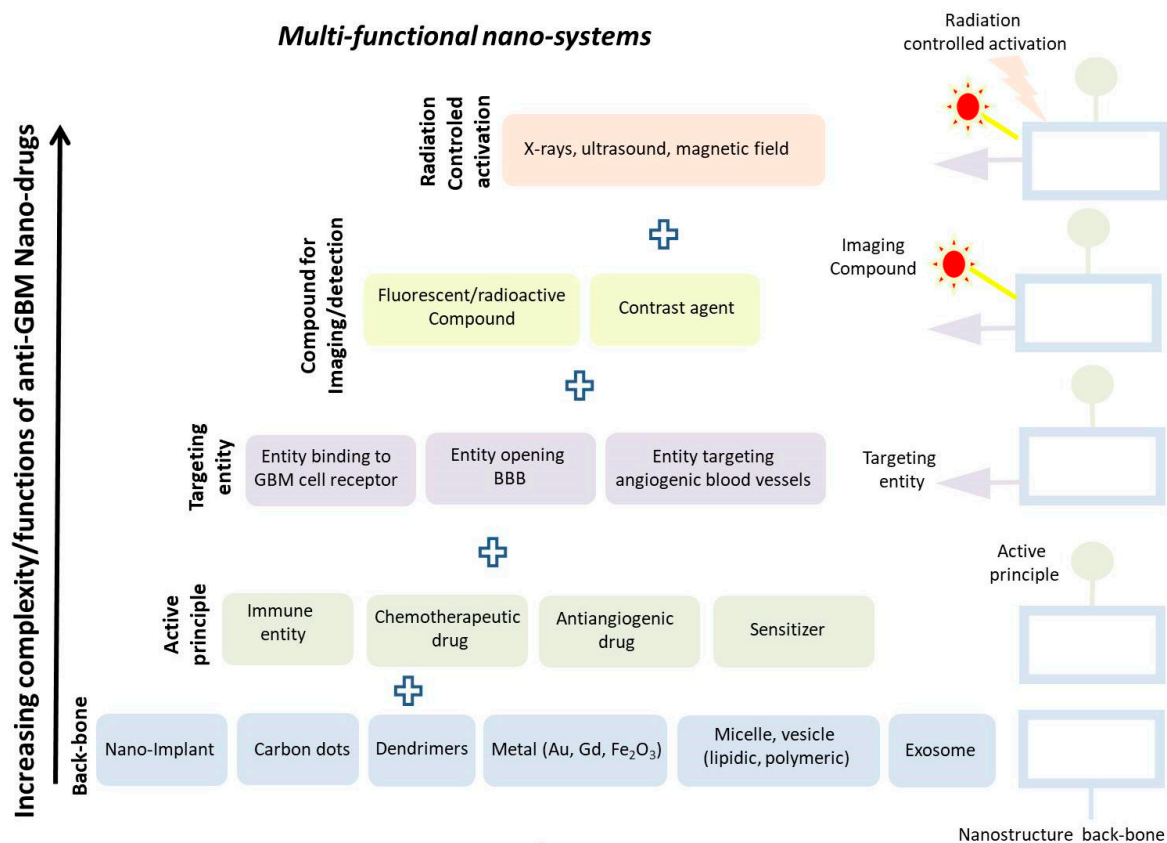
Figure 1. A schematic showing how a nanoparticulate system can be built up to include various functionalities to fight against GBM disease, such as: (i) a backbone, (ii) an active principle, (iii) a targeting moiety, and (iv) a compound used for imaging/detection.
