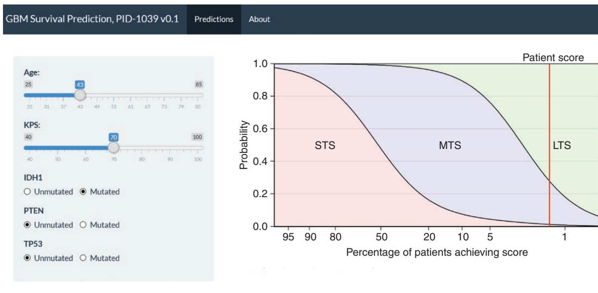
Figure 2. The application for GBM survival prediction using the survival-predictive nomogram. A representative clinical example is shown in which a 43-year-old GBM patient with a KPS score of 70 had an IDH1-mutant tumor. This patient had a 2%, 72%, and 26% chance of being a short-term survivor (<6 months), long-term survivor (>5 years), and median-term survivor (~15 months), respectively. Two percent of patients had this outcome.
