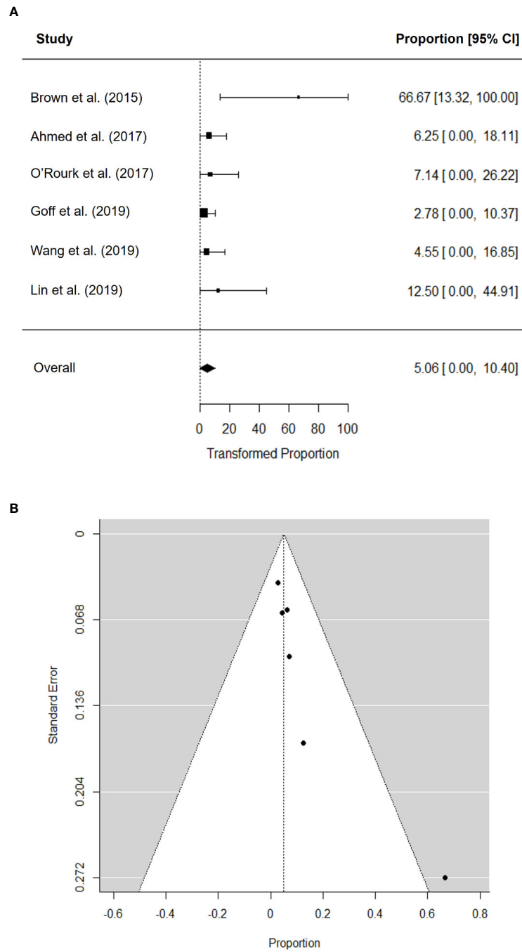
FIGURE 2 | Forest plot for objective response rate (A) and funnel plot of publication bias in objective response rate (B).
